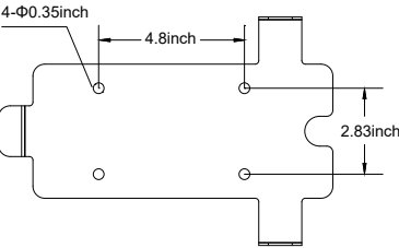
Wall-Mounted Bracket
